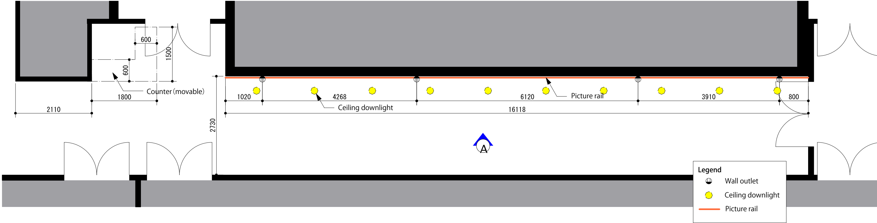
Floor plan S=1/60
