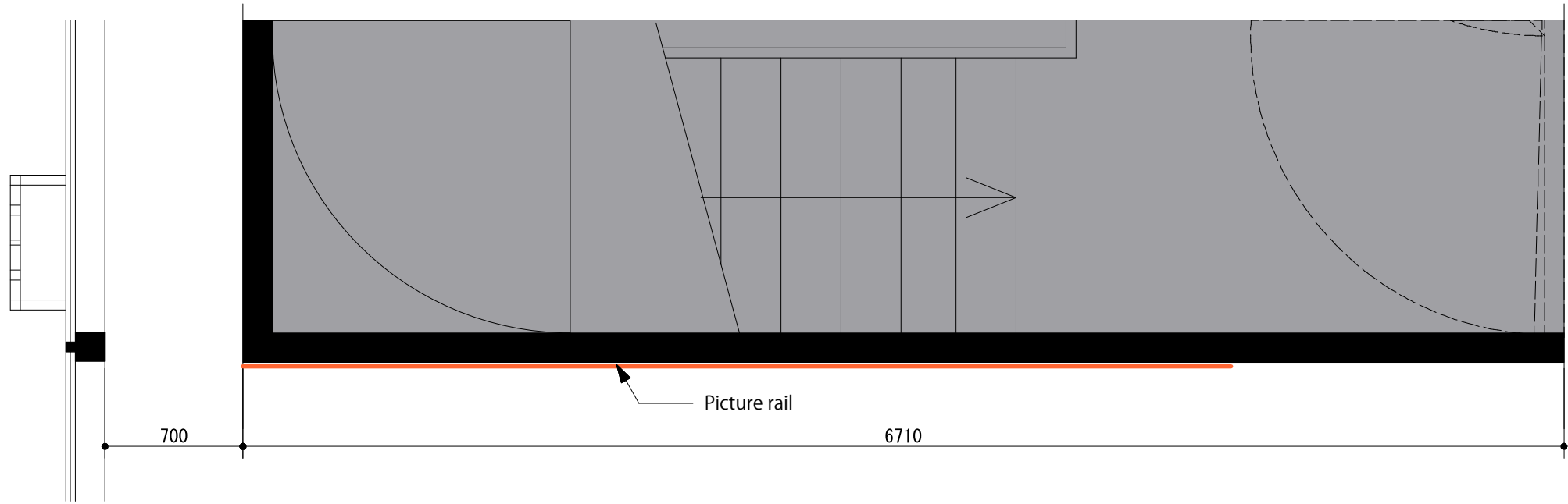
Floor plan S=1/30
